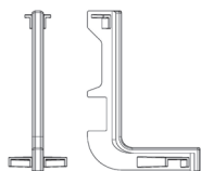
81/G11.A90B 90° INTERIOR
